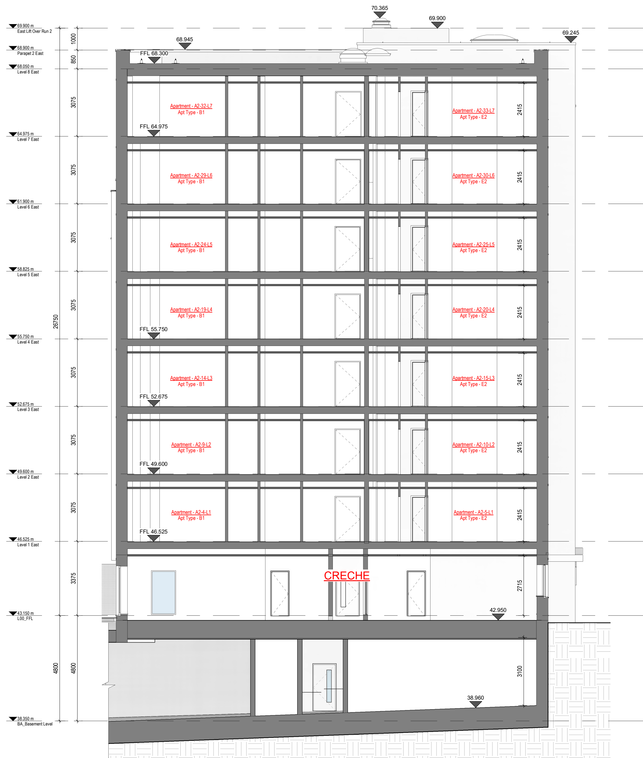
2 GA - Section BB
