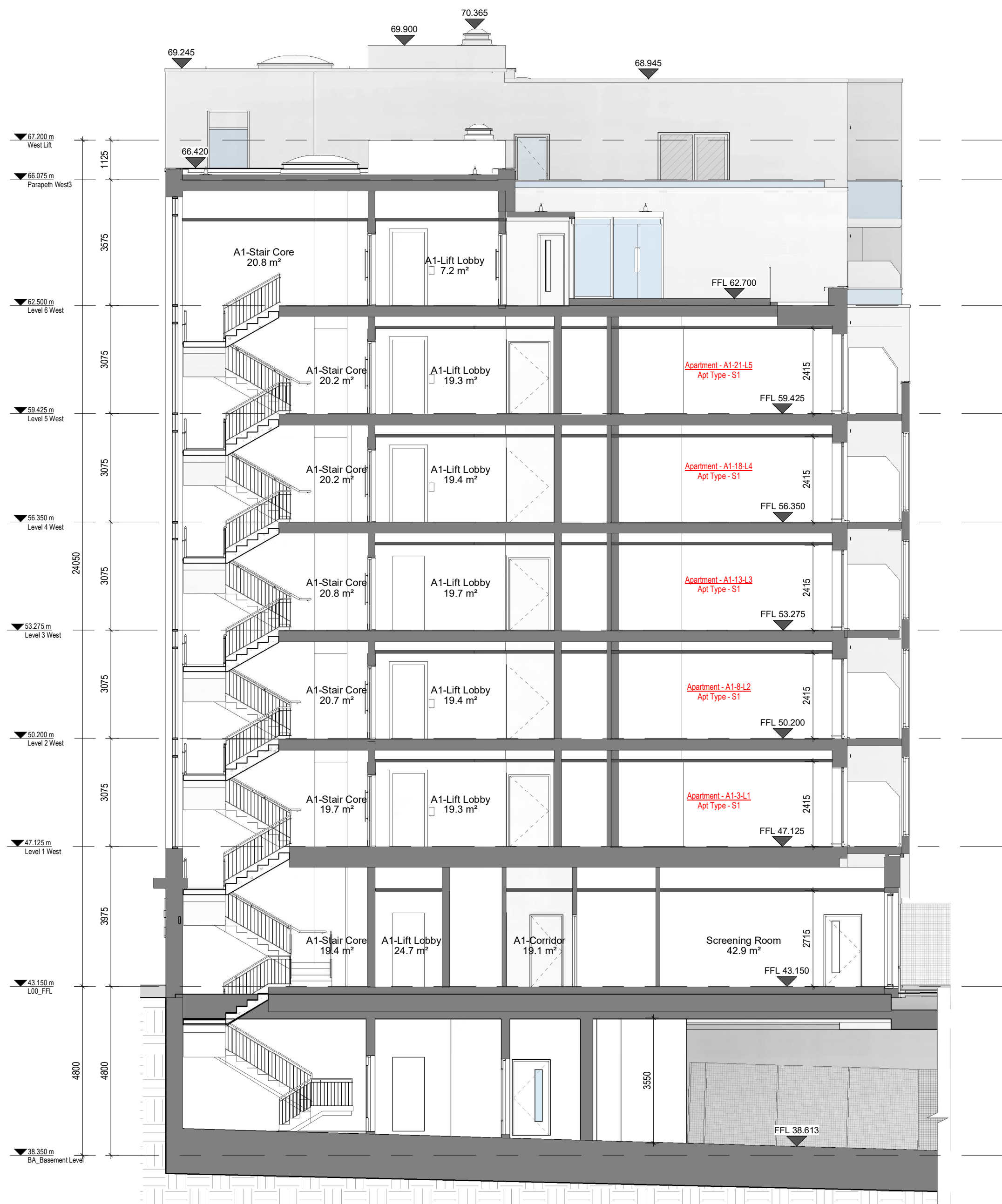
1 GA - Section AA
