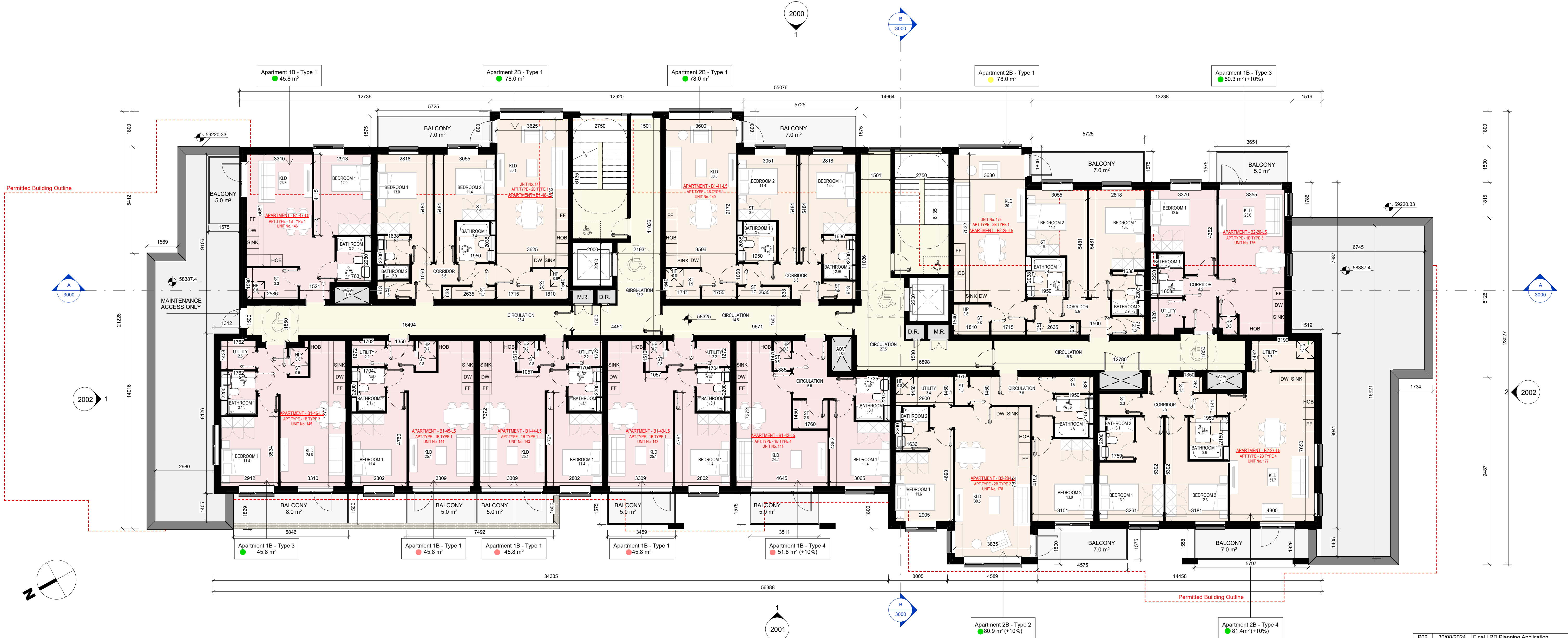
1 BLOCK B - L05- PROPOSED FIFTH FLOOR GA PLAN 1 : 100
