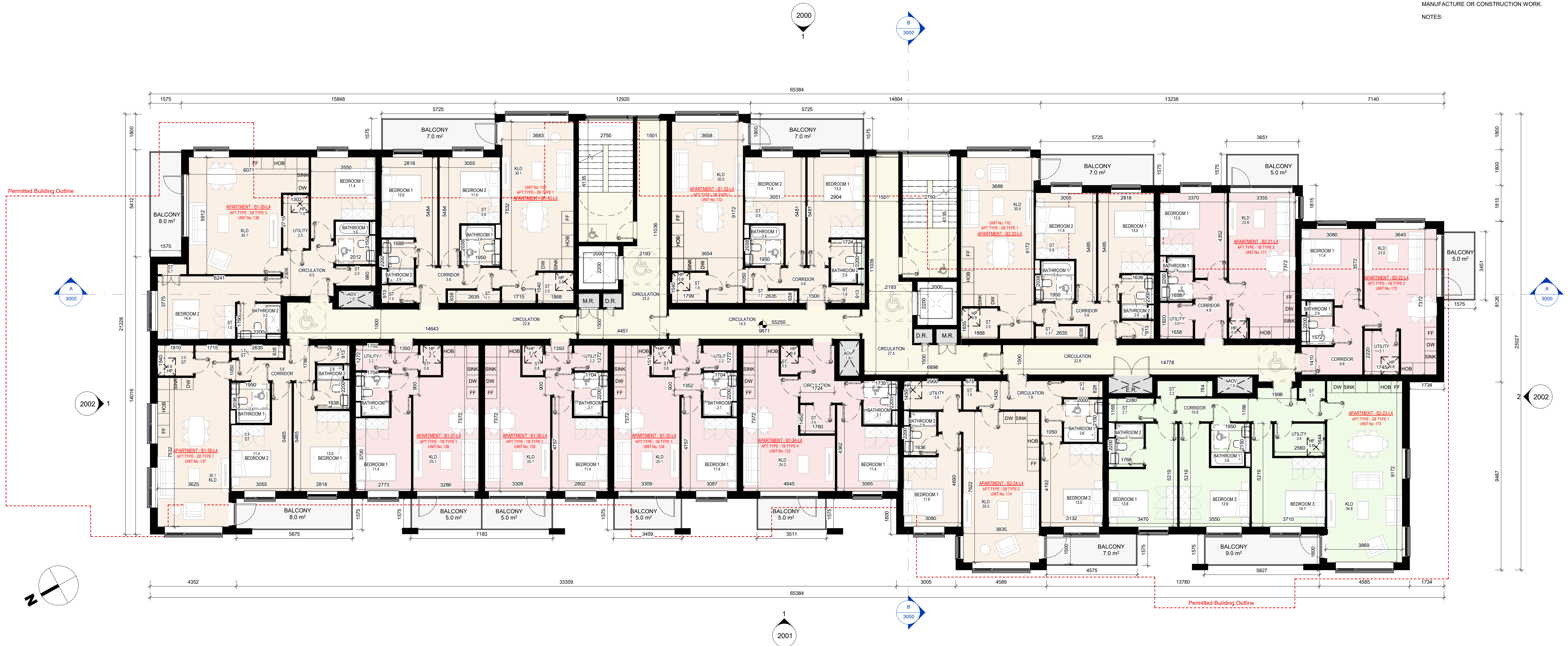
1 BLOCK B - L04- PROPOSED FOURTH FLOOR GA PLAN 1 : 100
