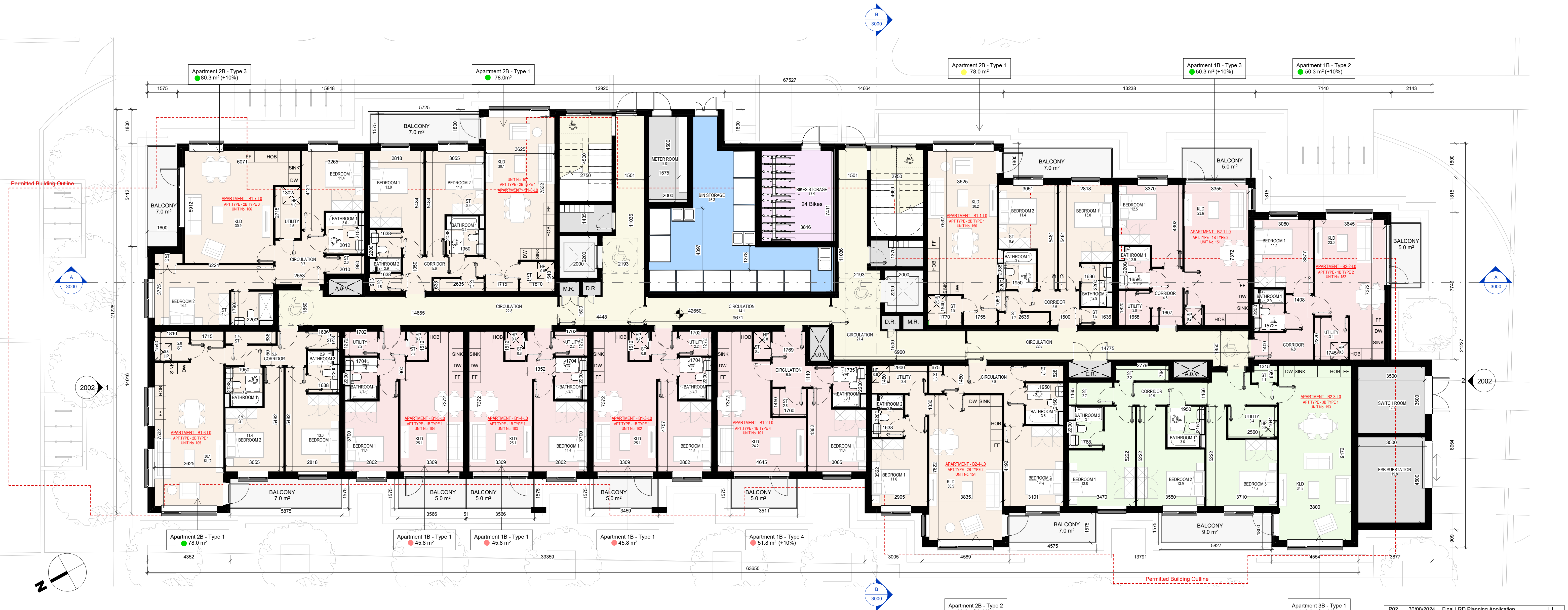
1 BLOCK B - L00- PROPOSED GROUND FLOOR GA PLAN
