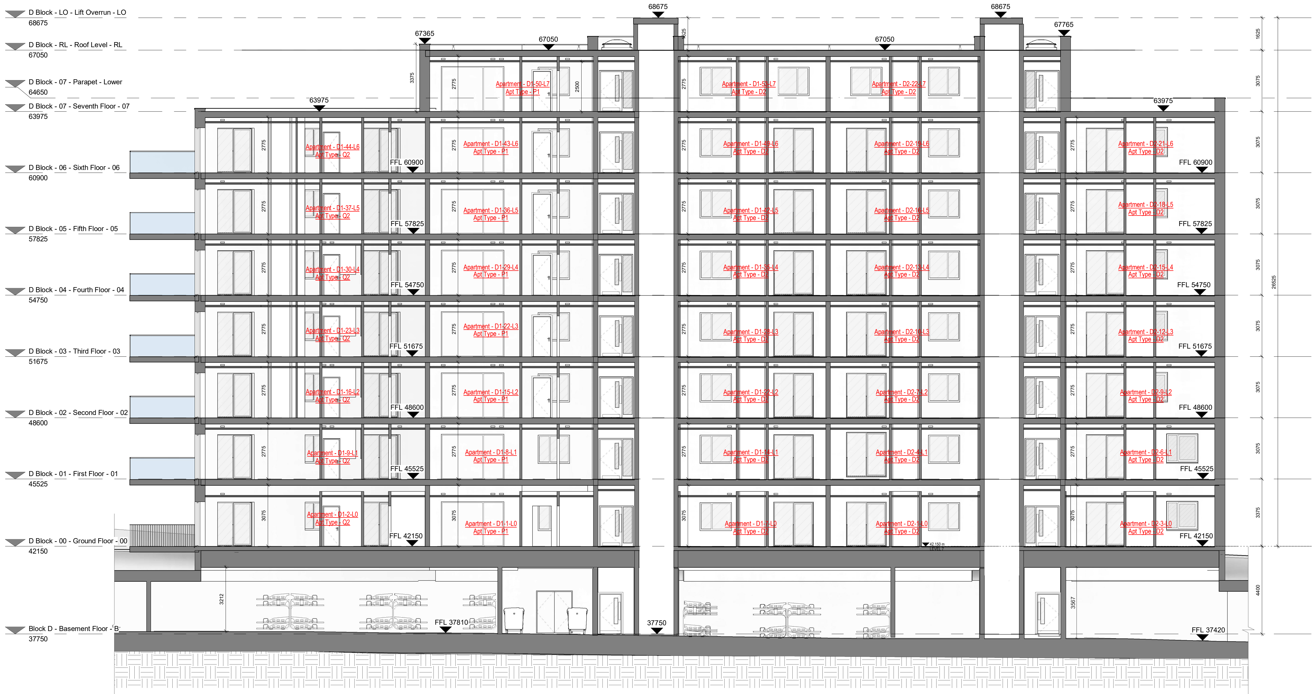
1 GA - Section AA
