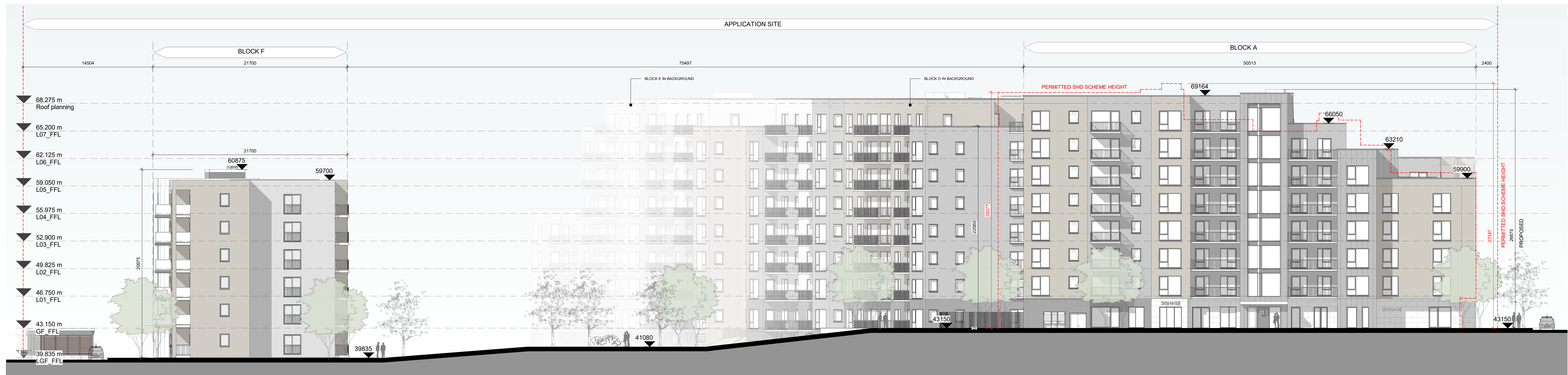
2 PROPOSED CONTEXTUAL ELEVATION - NORTH 1:200
