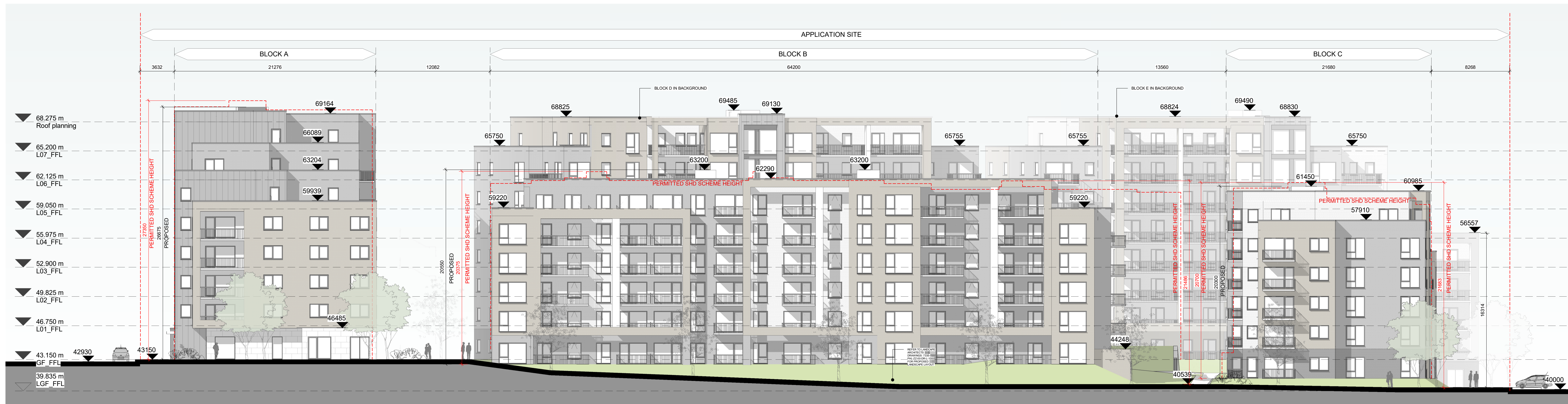
1 PROPOSED CONTEXTUAL ELEVATION - WEST 1:200
