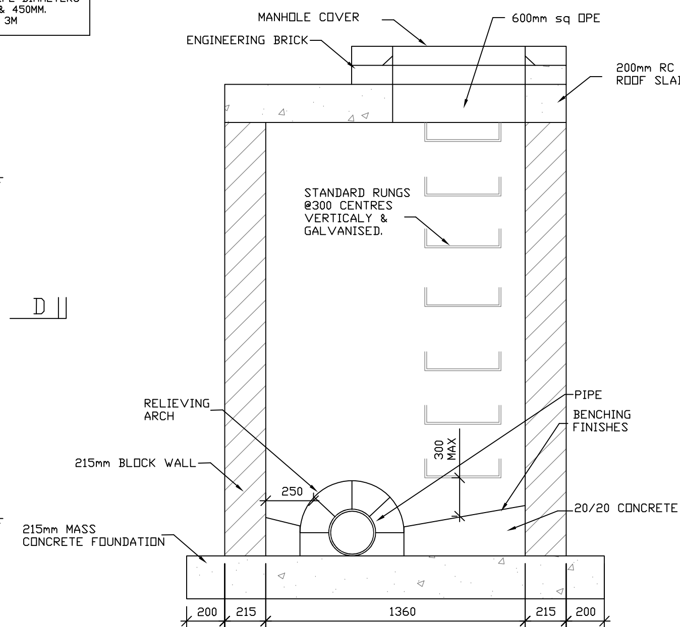
SECTION C-C SCALE 1:20
