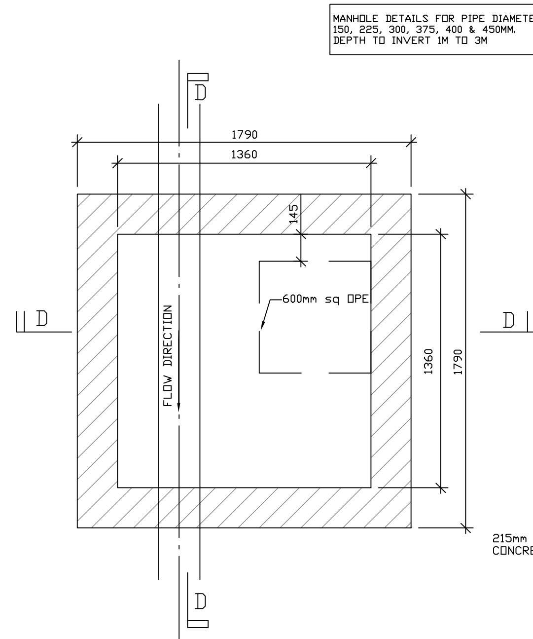
GDR TYPE MANHOLE TYPICAL DETAIL (DEPTH GREATER THAN 1M) SCALE 1:20
