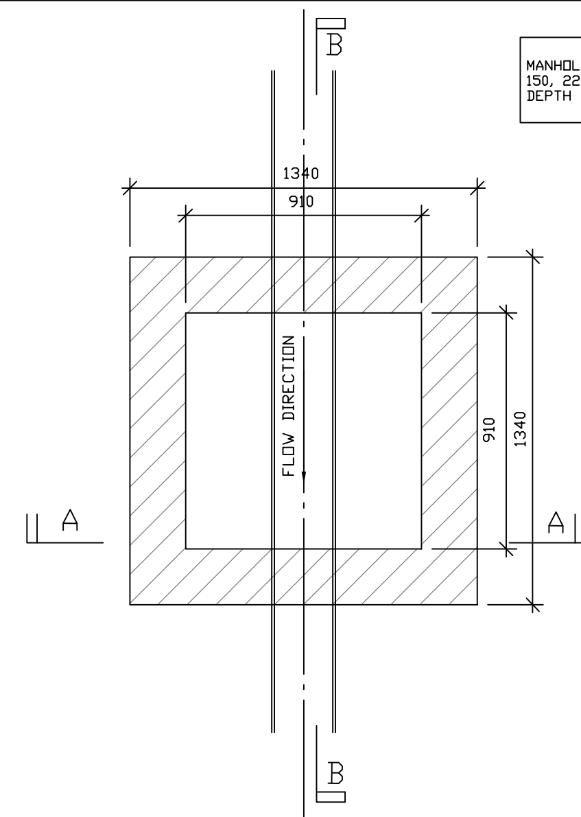
GDR TYPE MANHOLE TYPICAL DETAIL (DEPTH LESS THAN 1M) SCALE 1:20
