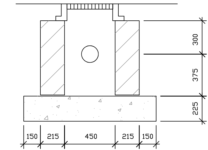
TYPICAL GULLY SECTION SCALE 1:20
