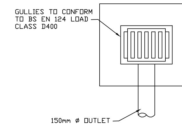
TYPICAL GULLY PLAN SCALE 1:20
