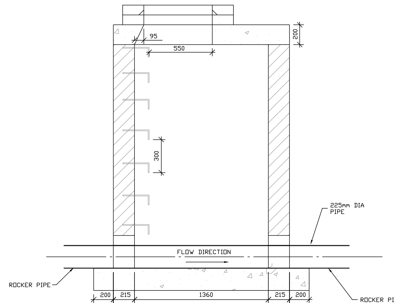
SECTION D-D SCALE 1:20
