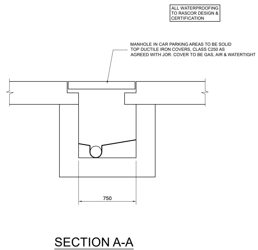
BASEMENT DRAINAGE SHALLOW INSPECTION CHAMBER DETAIL (MAX 1m DEPTH TO INVERT)
