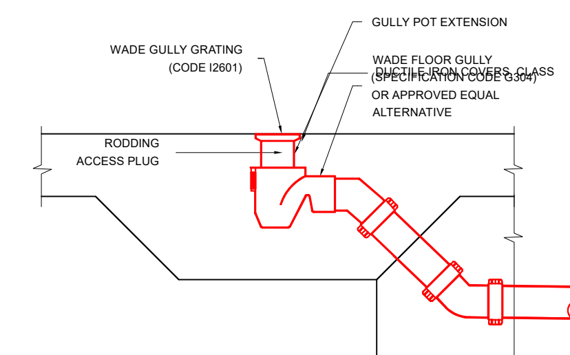
TYPICAL PAVING GULLY DETAILS
