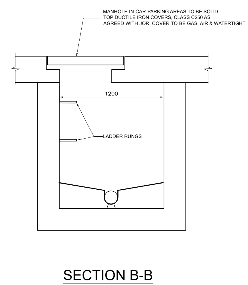
BASEMENT DRAINAGE DEEP MANHOLE CHAMBER DETAIL (MAX 3m DEPTH TO INVERT)
