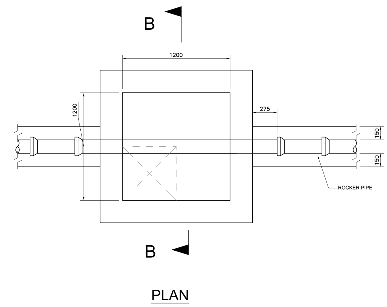
BASEMENT DRAINAGE DEEP MANHOLE CHAMBER DETAIL (MAX 3m DEPTH TO INVERT)
